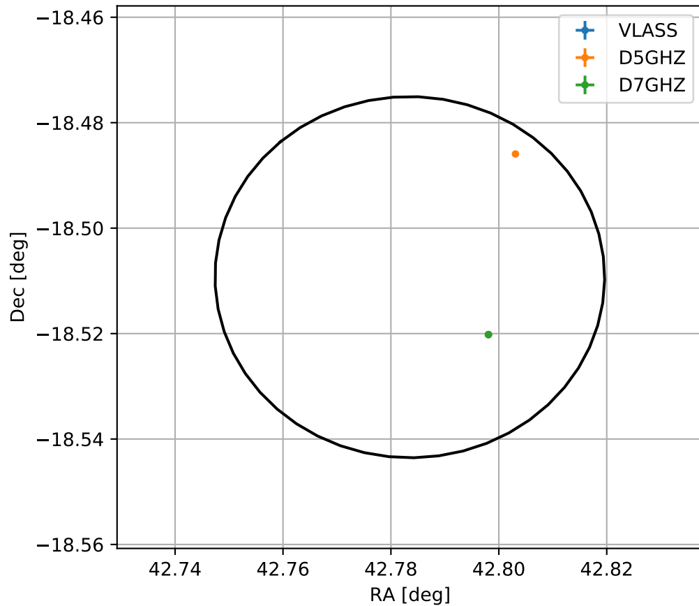
4FGL J0251.1-1830
