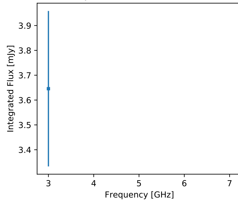
F357 J024020.10-024702.2 (unr)
