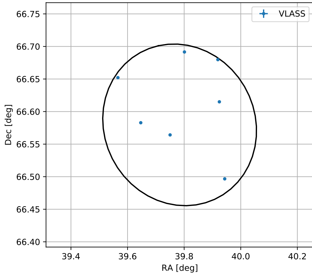
4FGL J0239.1+6634
