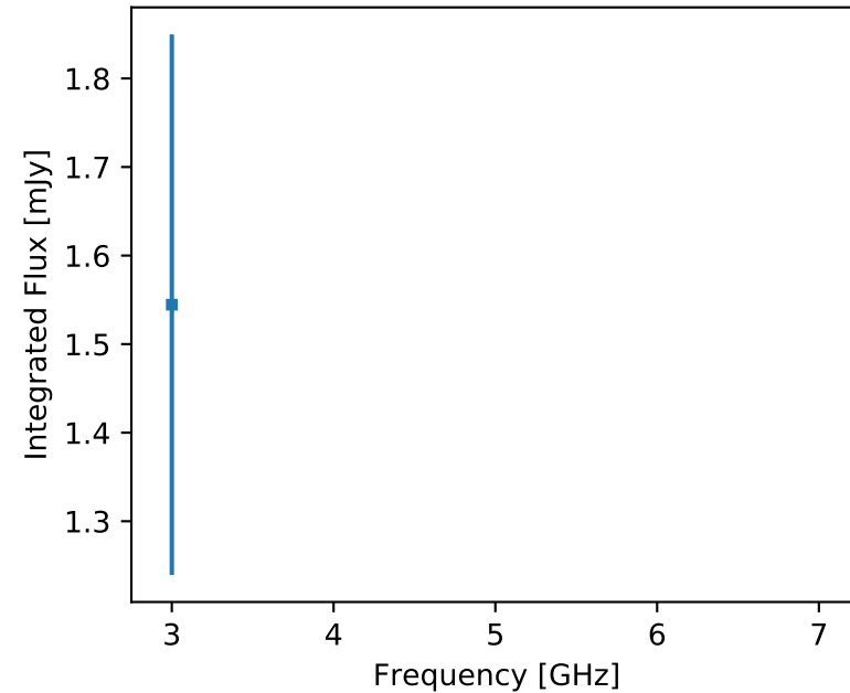
F357 J023810.56-262608.5 (unr)
