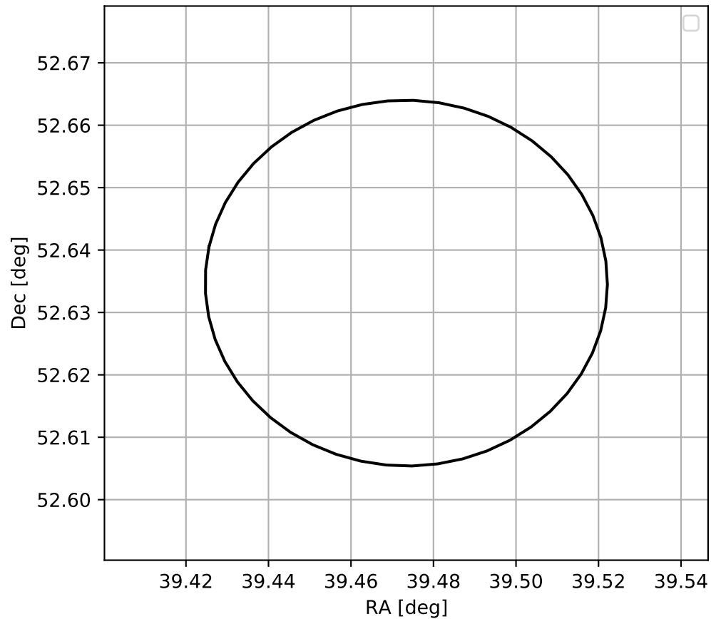
4FGL J0237.8+5238
