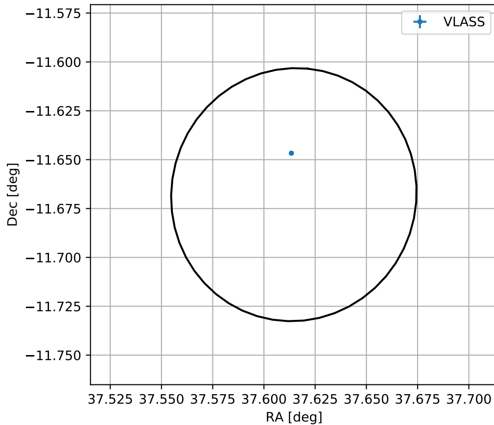
4FGL J0230.4-1140
