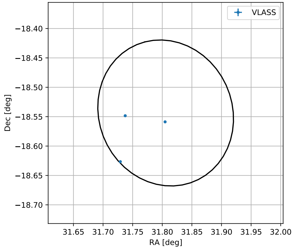
4FGL J0207.2-1832
