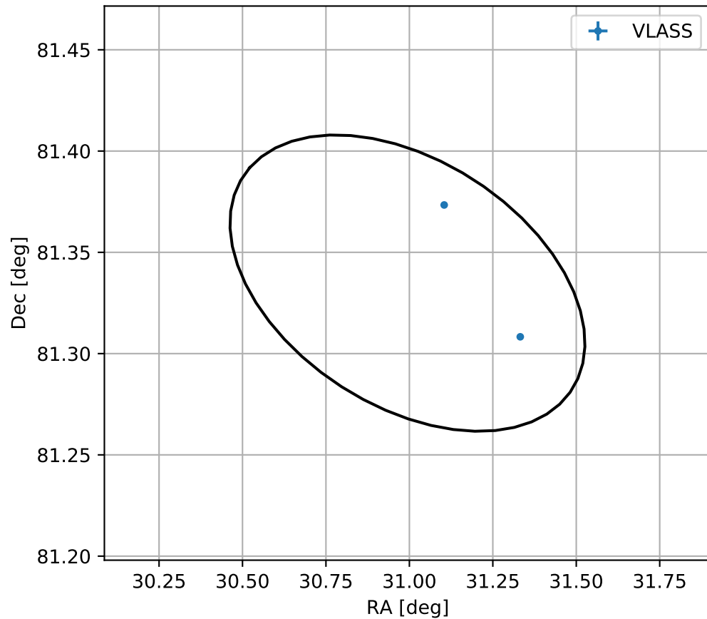
4FGL J0203.9+8120
