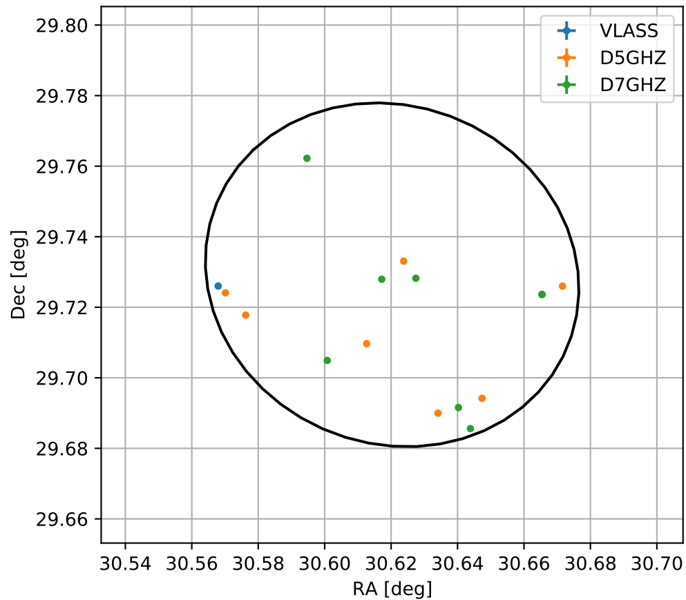
4FGL J0202.4+2943
