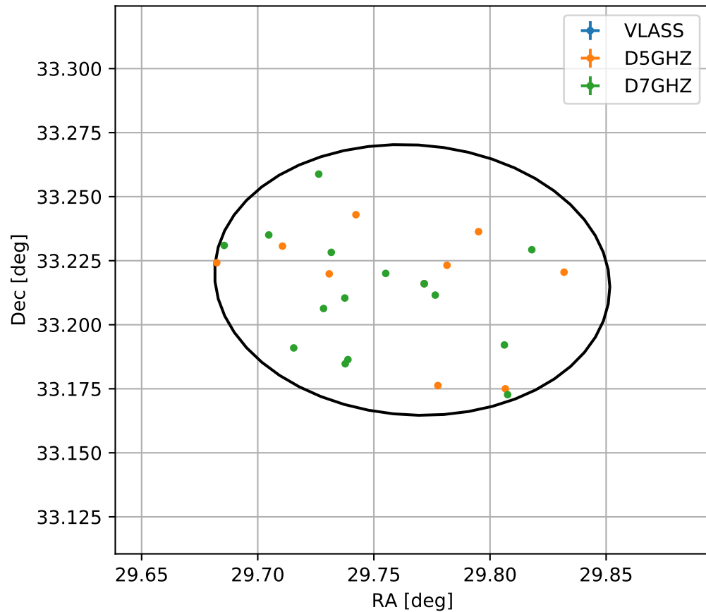
4FGL J0159.0+3313
