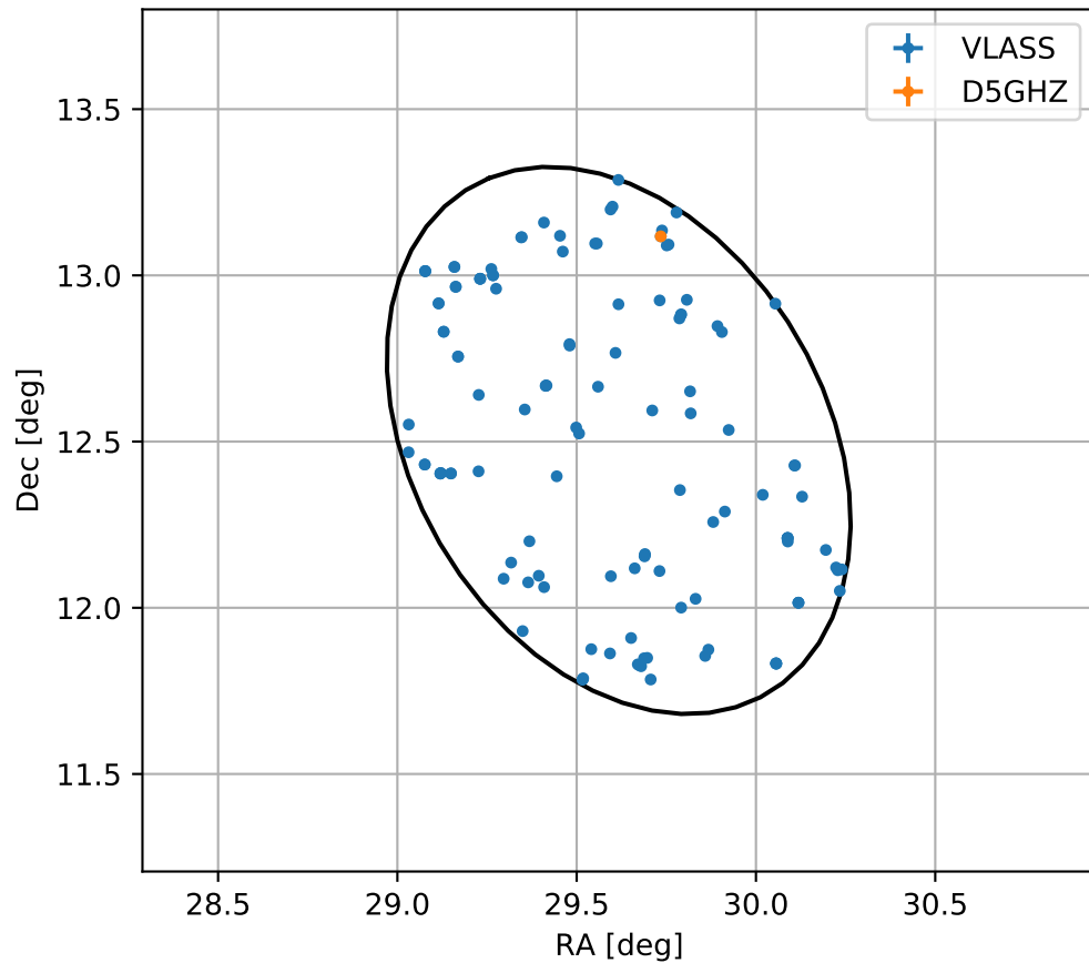
4FGL J0158.4+1230
