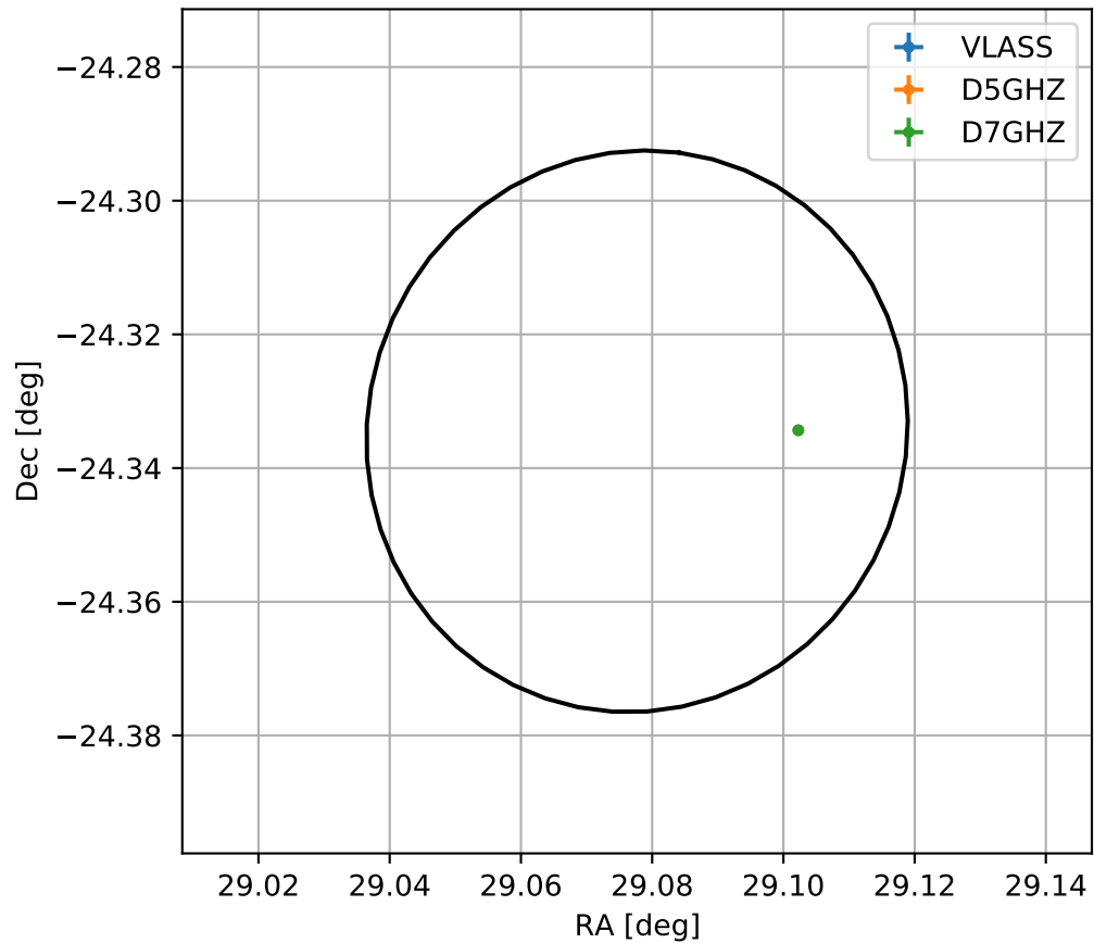
4FGL J0156.3-2420
