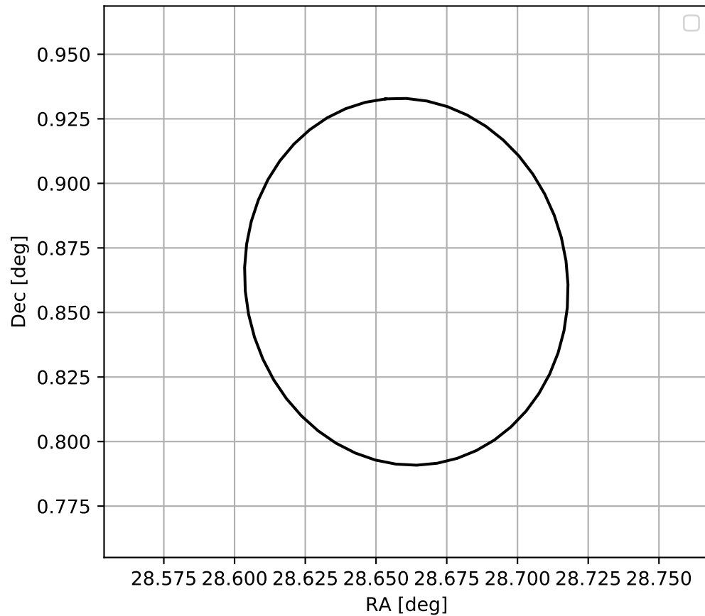
4FGL J0154.6+0051
