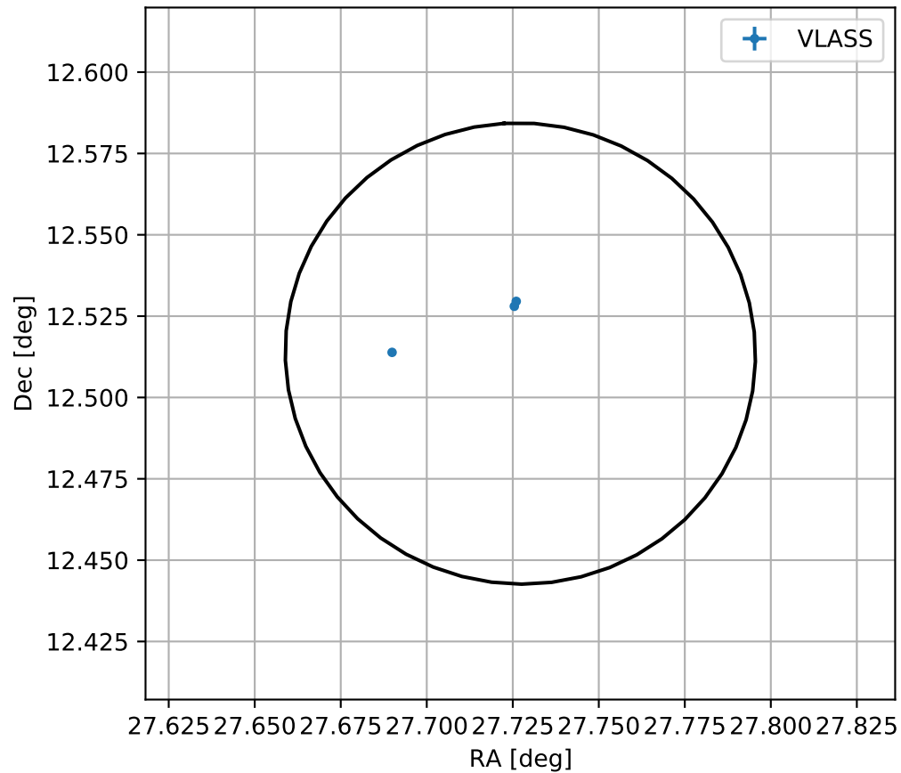
4FGL J0150.9+1230
