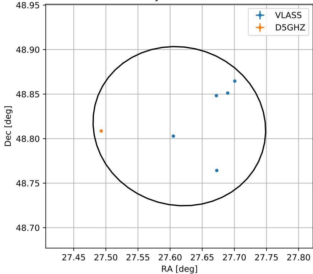
4FGL J0150.4+4848
