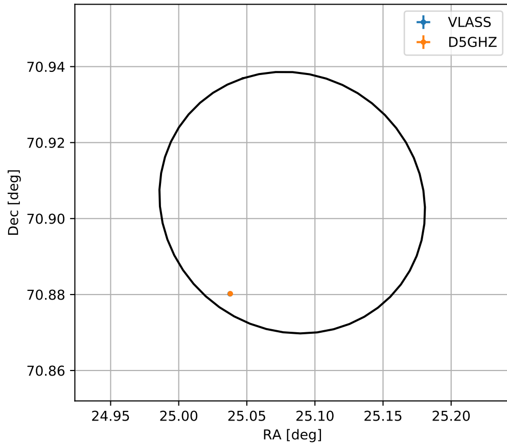
4FGL J0140.3+7054
