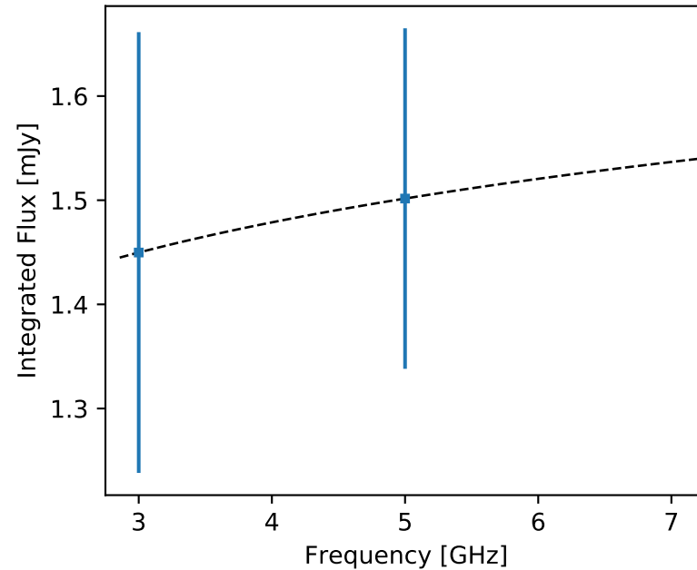
F357 J014009.08+705248.8 (unr)
