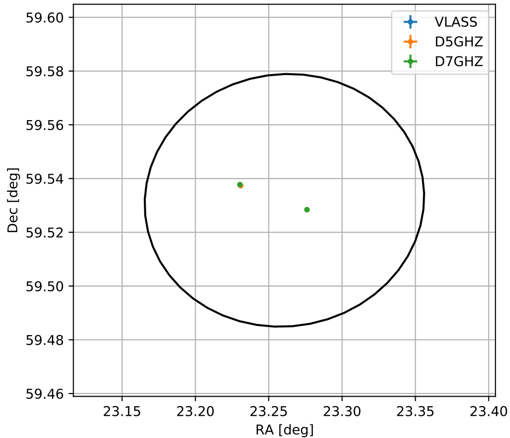
4FGL J0133.0+5931
