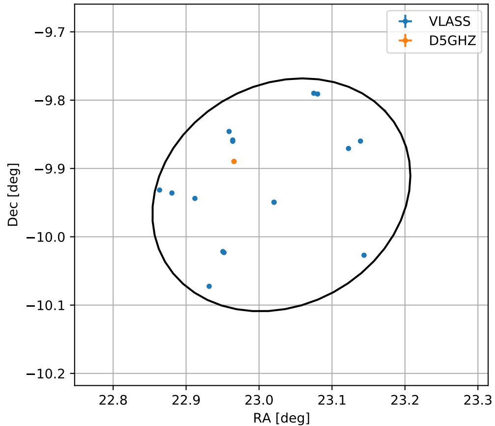
4FGL J0132.1-0956
