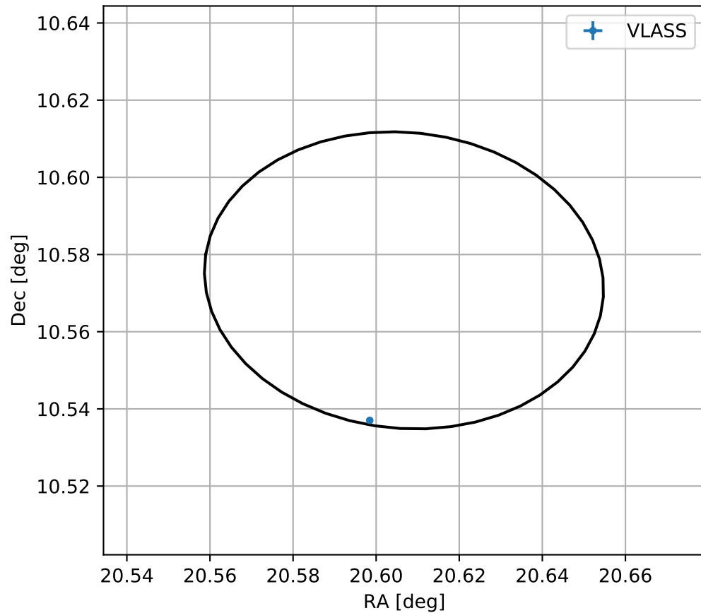
4FGL J0122.4+1034
