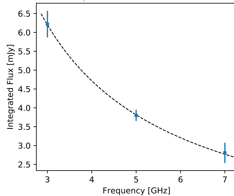
F357 J011528.95-291844.2 (unr)
