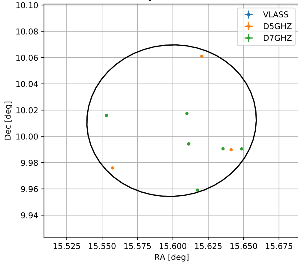
4FGL J0102.3+1000
