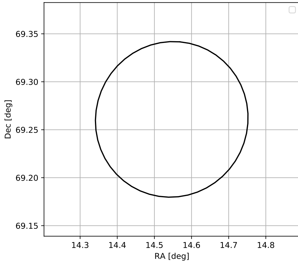
4FGL J0058.1+6915
