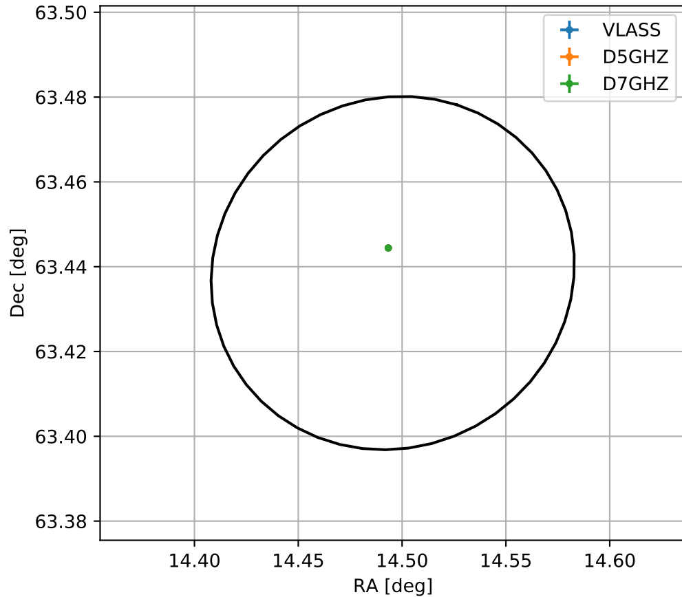
4FGL J0057.9+6326
