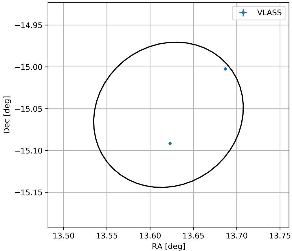
4FGL J0054.4-1503
