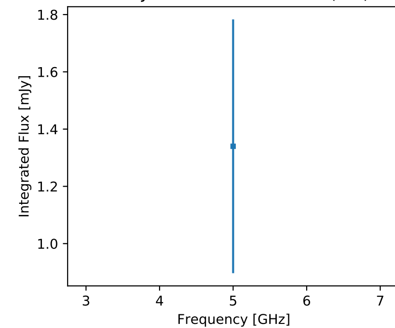
F357 J005222.84+644916.4 (unr)
