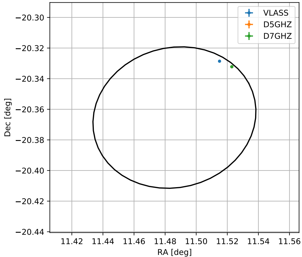
4FGL J0045.9-2021
