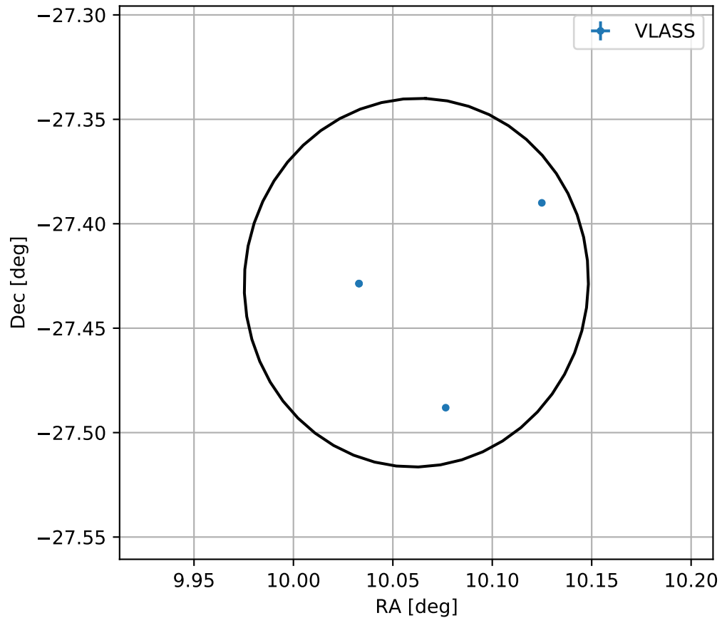
4FGL J0040.2-2725
