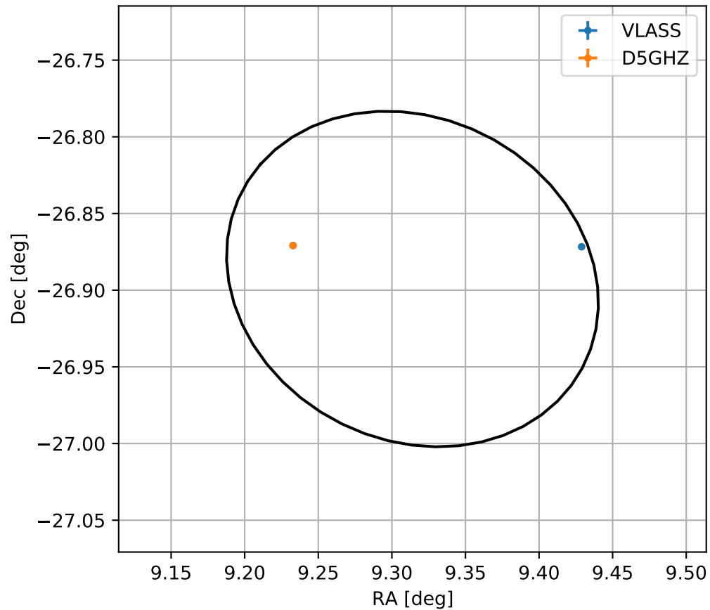
4FGL J0037.2-2653
