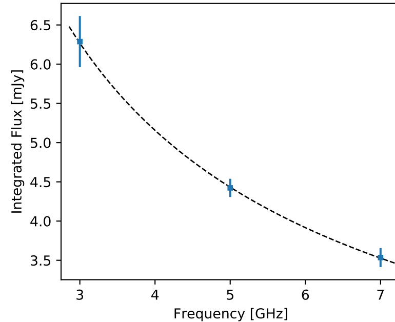
F357 J003514.80-174019.7 (unr)
