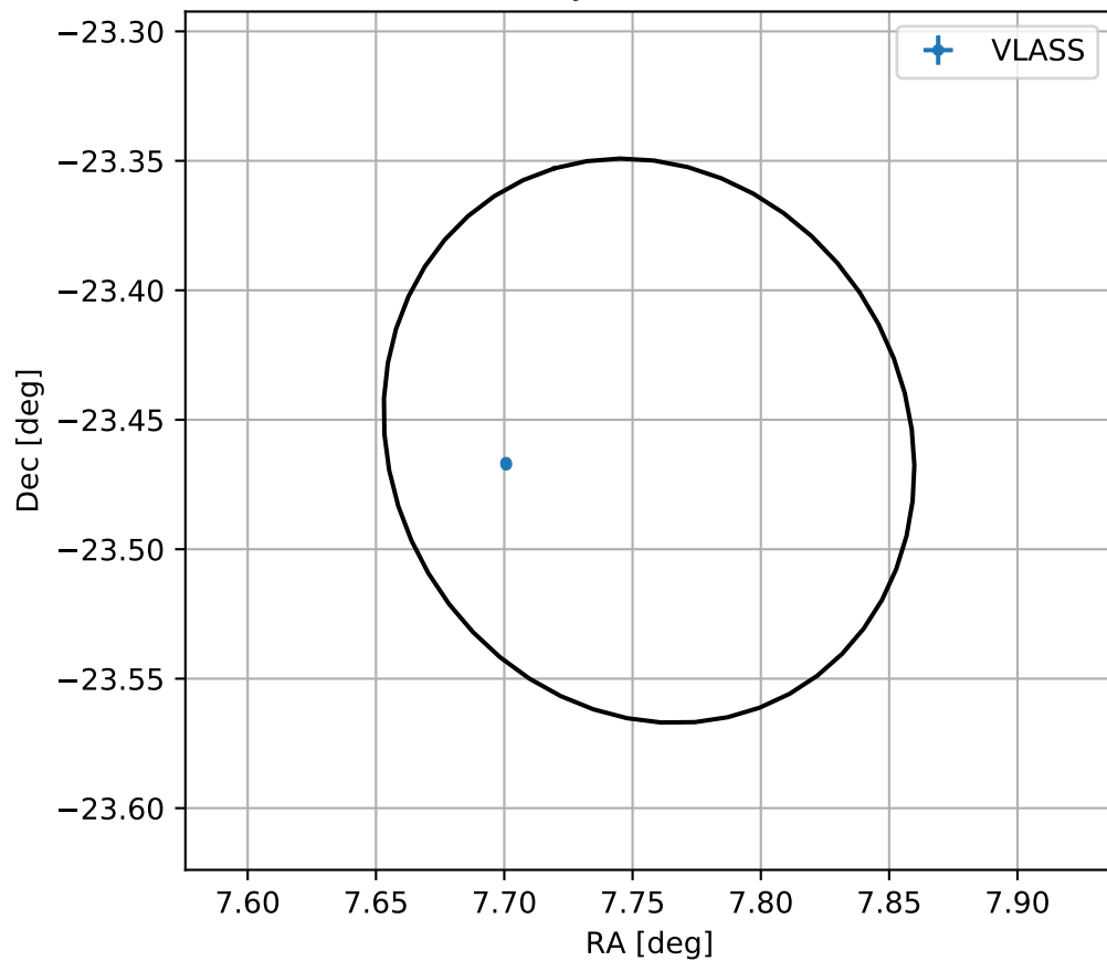
4FGL J0031.0-2327
