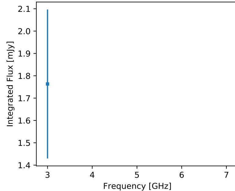
F357 J003048.18-232802.4 (res)
