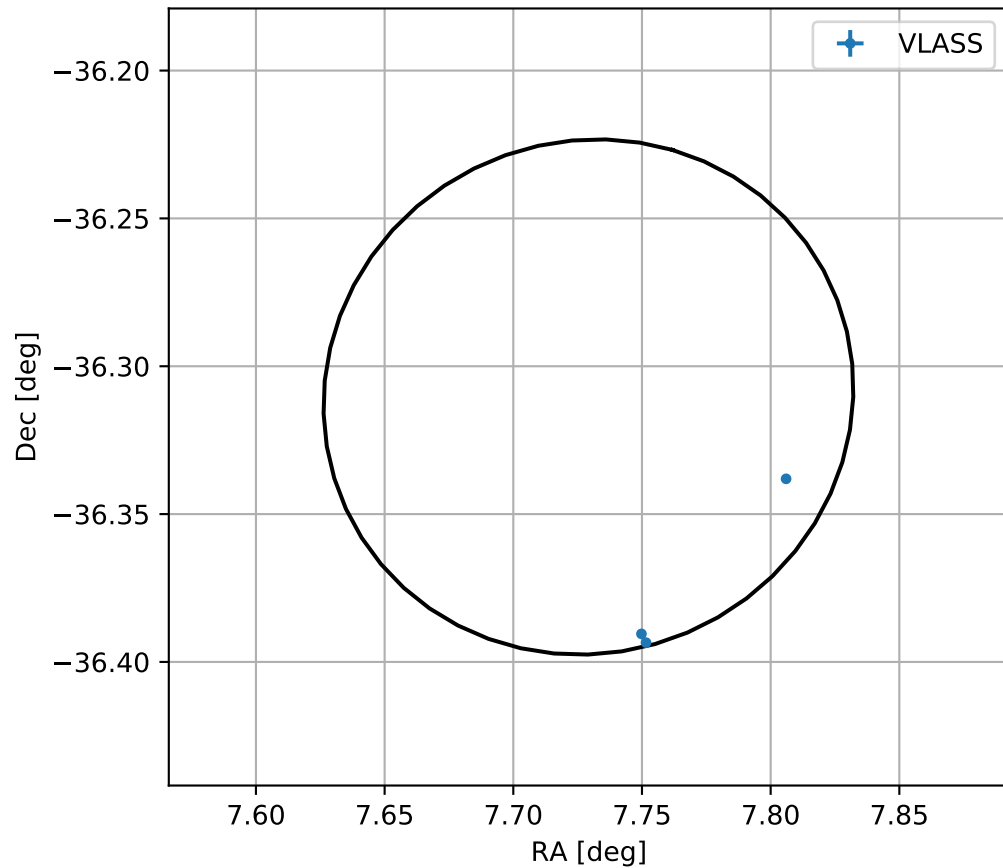
4FGL J0030.9-3618
