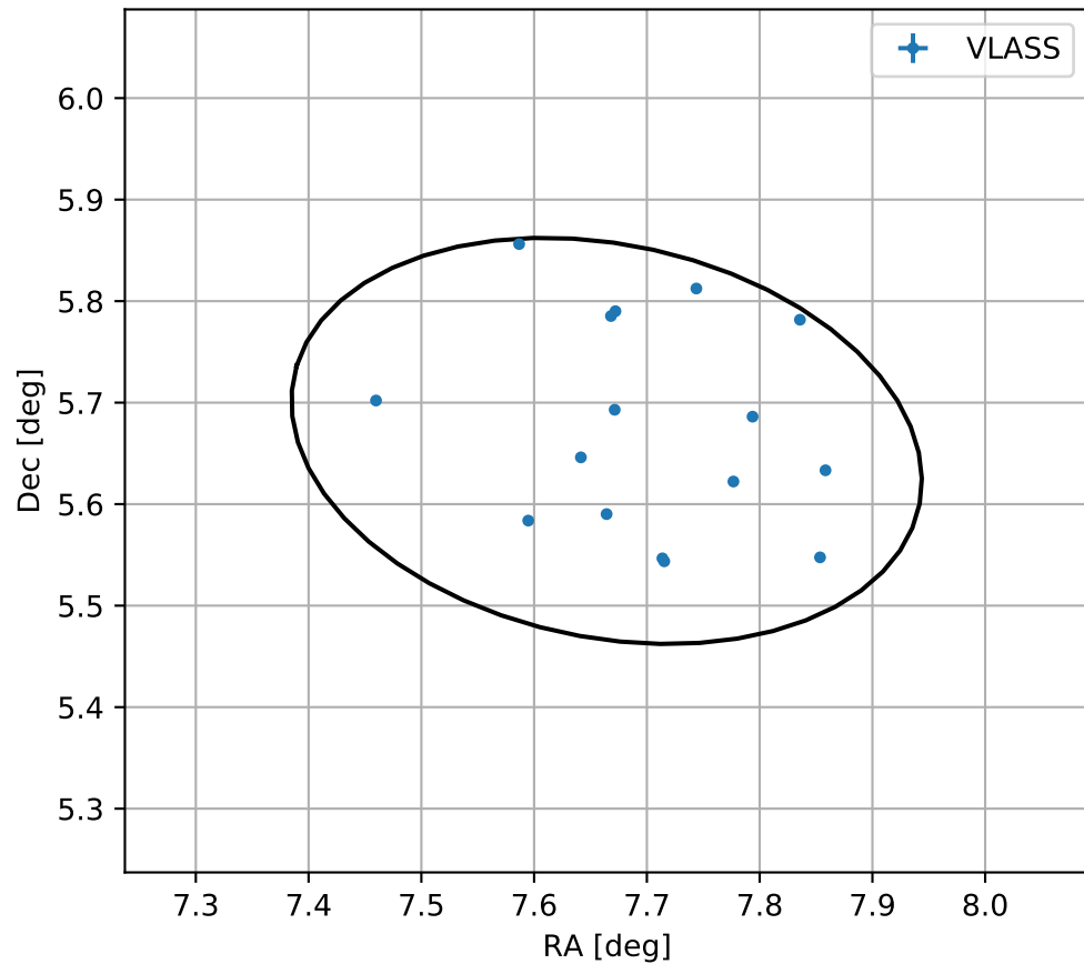
4FGL J0030.6+0539
