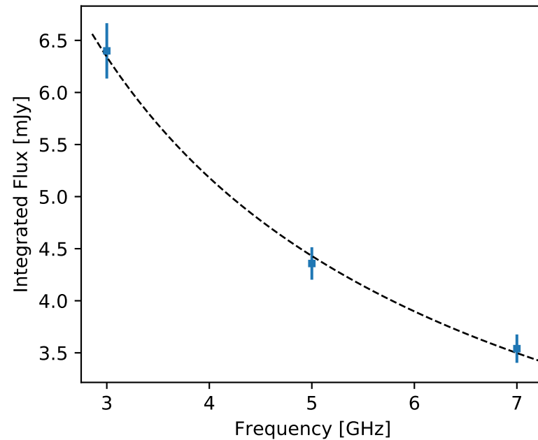
F357 J002611.63-073115.8 (unr)
