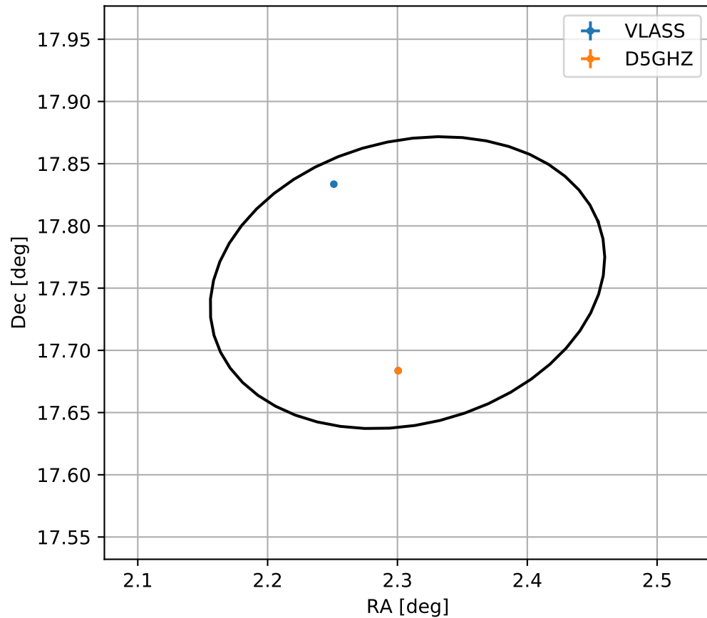
4FGL J0009.2+1745
