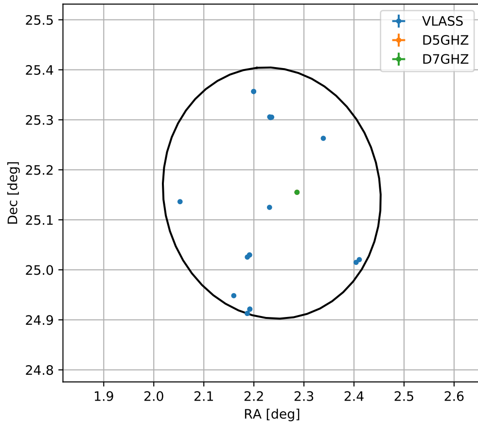
4FGL J0008.9+2509
