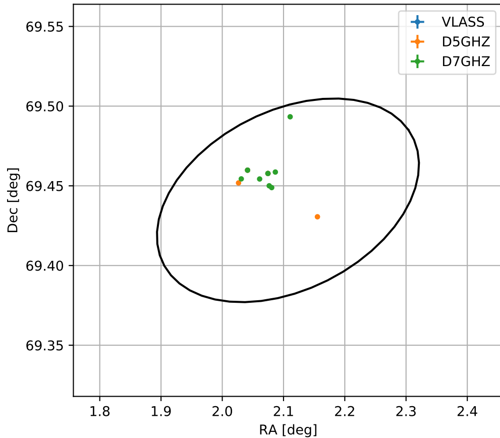
4FGL J0008.4+6926
