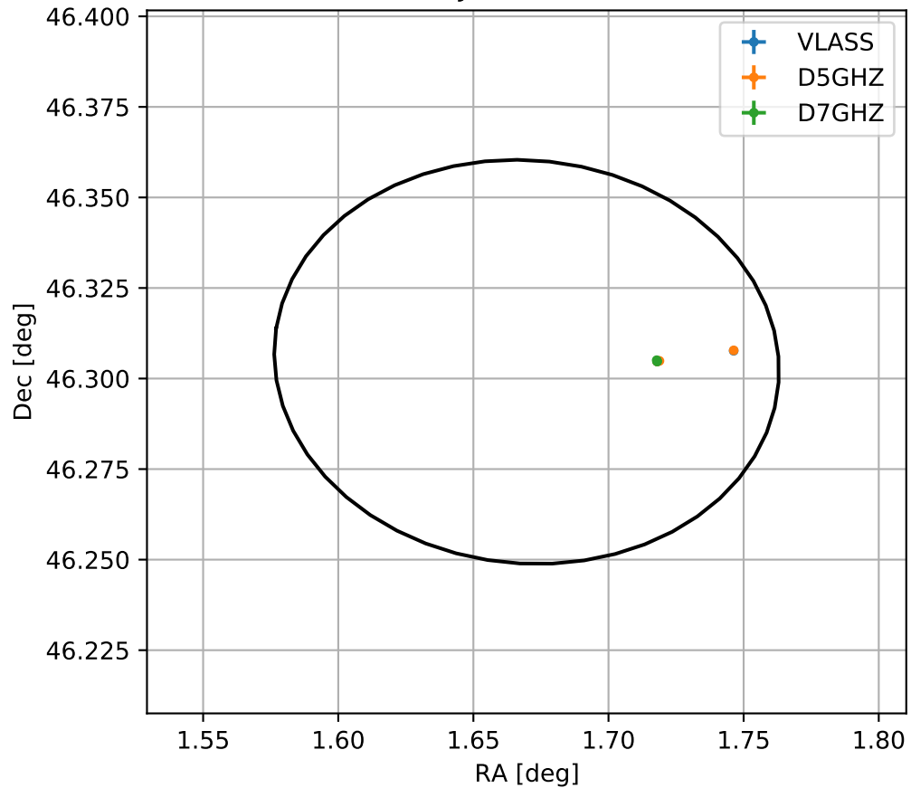
4FGL J0006.6+4618
