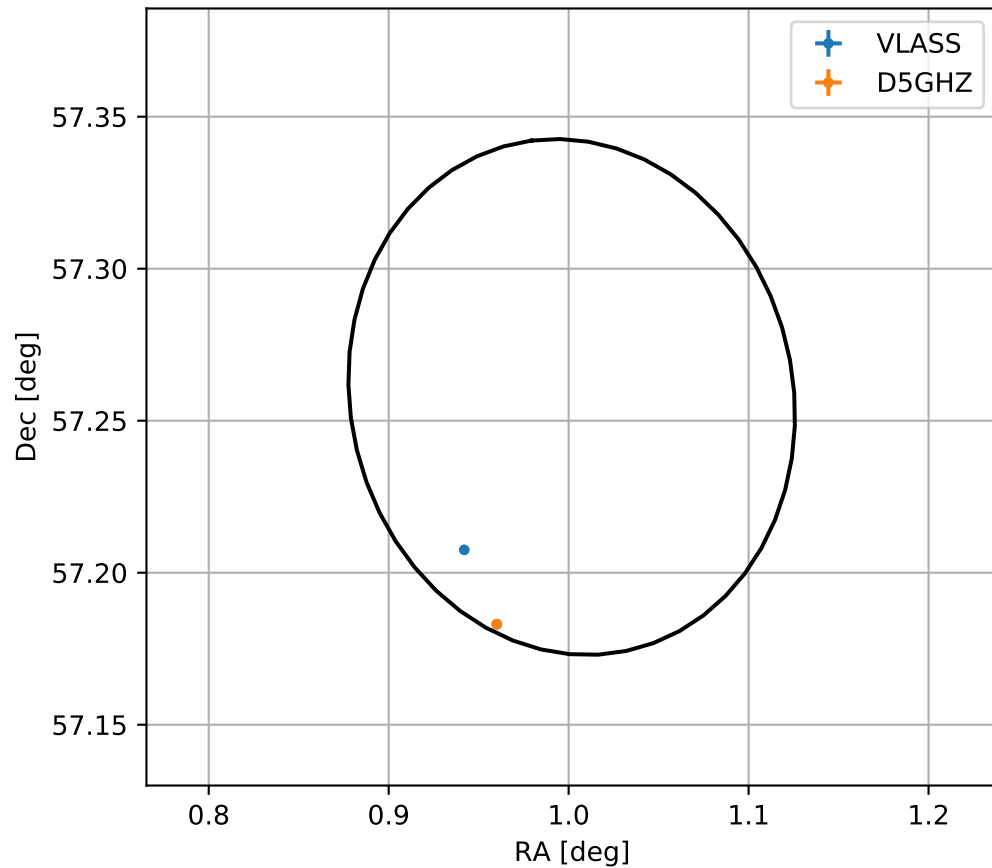
4FGL J0004.0+5715
