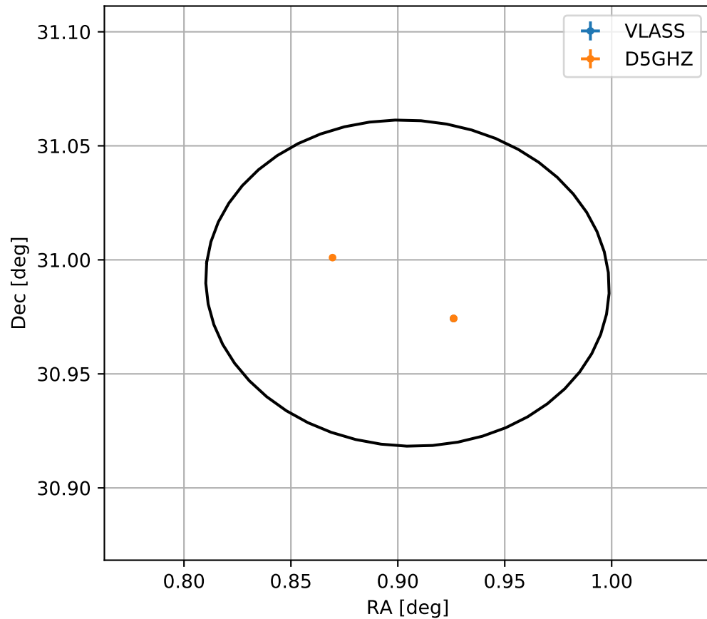
4FGL J0003.6+3059
