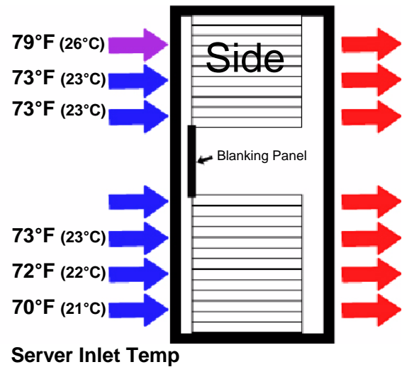
2B: With airflow management blanking panels
