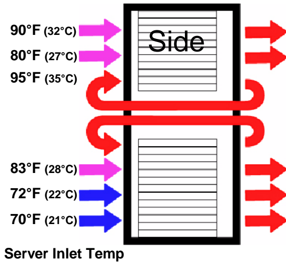
2A: Without airflow management blanking panels
