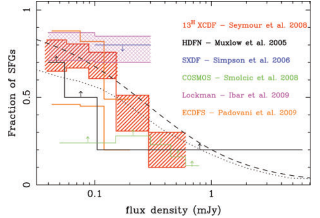
Figure 4 Differential fraction of star-forming galaxies as a function of 1.4 GHz flux density, from a selection of recent deep surveys. Shaded boxes, and the two lines for Padovani et al., show the range of uncertainty in the survey results. Arrows indicate constraints from other surveys. These results show that the fraction of star-forming galaxies increases rapidly below 1 mJy and, at the 50 \mu Jy survey limit of EMU, about 75% of sources will be star-forming galaxies.
