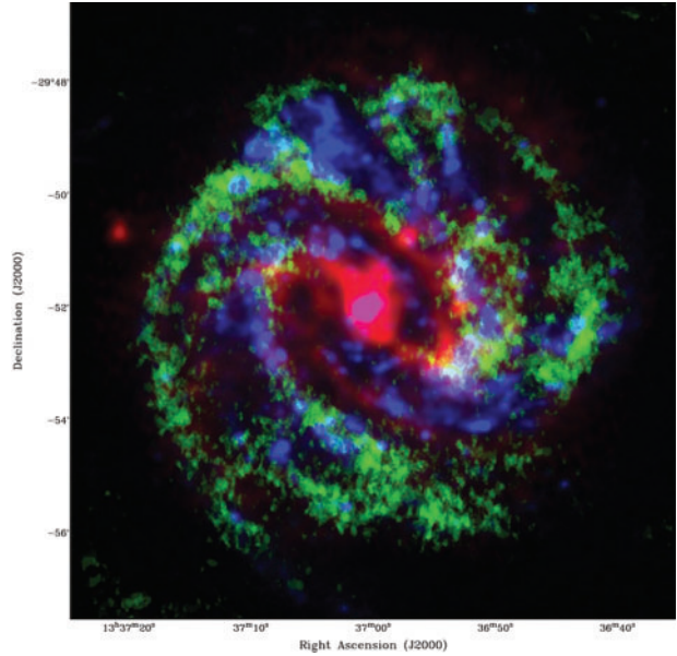
Figure 8 This multi-wavelength composite image of the inner part of the spiral galaxy M83 highlights the synergy between the two key ASKAP large survey science projects: WALLABY and EMU. The ATCA 20-cm radio continuum emission is shown in red, the ATCA HI distribution in green, and the GALEX FUV emission in blue (Koribalski et al. 2008; Gil de Paz et al. 2007).
