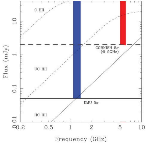
Figure 13 Spectral energy distribution of HII regions over the frequency ranges of the EMU & CORNISH surveys. The solid, dashed and dot-dashed lines represent the brightnesses of spherical isothermal and homogeneous hypercompact (HC), ultracompact (UC) and compact (C) HII regions at an assumed distance of 18 kpc. The red band shows the frequency range of the 5-GHz CORNISH survey and the blue band the range of the 1.3-GHz EMU survey. 5\sigma detection limits are indicated by horizontal lines.
