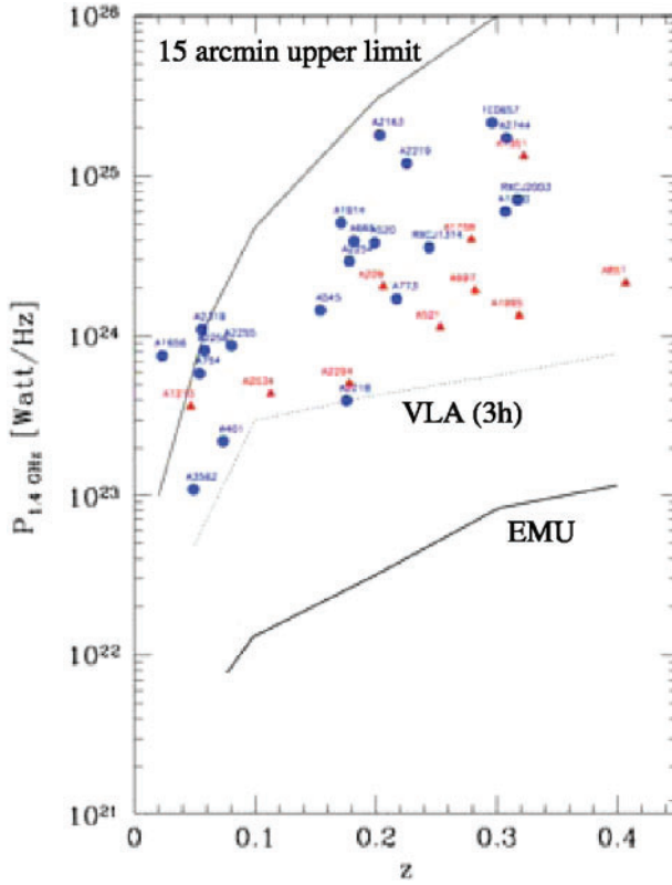
Figure 9 1.4 GHz radio power of detected cluster haloes as a function of redshift showing the detection limits of previous cluster observations, adapted from Giovannini et al. (2009), and the 5\sigma calculated detection limit of EMU, assuming a halo with a diameter of 1 Mpc, using the calculated ASKAP sensitivity on different scale sizes discussed in §1.2. The upper line shows the limit corresponding to a scale size of 15 arcmin, which is approximately the largest object that can be imaged with the VLA unless single-dish data are added to the interferometry data. At high redshifts, sensitivity may be limited by confusion, although we expect to overcome this by subtracting off compact sources.
