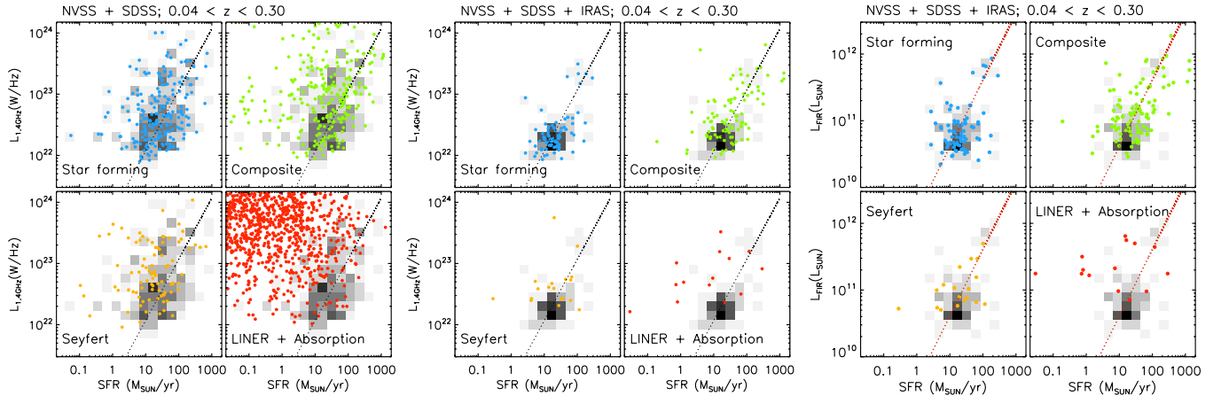
Figure 11. 1.4 GHz radio (left and middle panel) and FIR (right panel) luminosity as a function of SFR, derived via SED fitting to the NUV–NIR SDSS photometry (see the text for details). In the three large panels different galaxy types (symbols) and samples (indicated above and in each panel) are shown. The gray-scale histogram in each plot shows the distribution of star-forming galaxies for a given sample. Superimposed on the plots (dashed lines) are calibrations converting radio and FIR luminosity to SFR (Yun et al. 2001; Kennicutt 1998).
