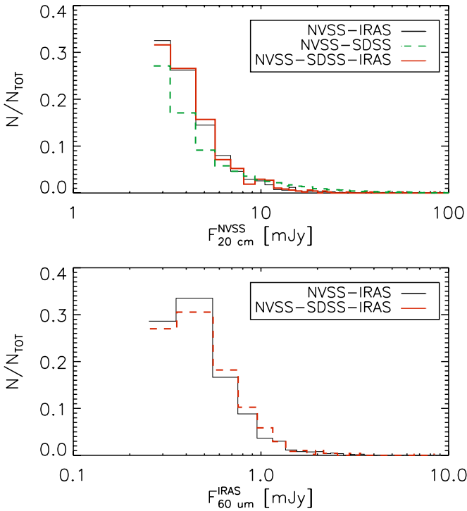
Figure 2. Distribution of flux density at 20 cm (top panel) and 60 \mu m (bottom panel) for various radio-selected samples indicated in the top right of the panels. (A color version of this figure is available in the online journal.)
