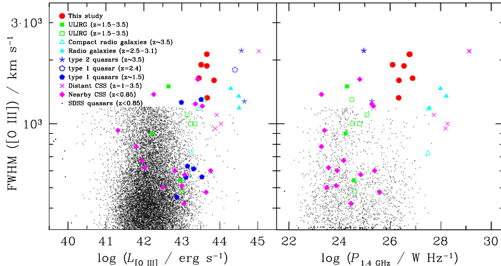
Figure 3. Left: FWHM of [O III] vs. [O III] luminosity for our sample (red circles) and various types of AGNs: high- z ULIRGs (green squares; Harrison et al. 2012), high- z radio galaxies (cyan triangles; Nesvadba et al. 2007, 2008), high- z type 2 quasars (blue solid stars; Nesvadba et al. 2011), high- z type 1 quasars (blue pentagons; Ho et al. 2012; Cano-Díaz et al. 2012), high- z compact steep-spectrum (CSS) sources (magenta crosses; Hirst et al. 2003), nearby CSS sources (magenta diamonds; Gelderman & Whittle 1994), and nearby type 1 quasars from SDSS (small black dots; Shen et al. 2011). The FWHMs are derived either from single-Gaussian (filled symbols) or double-Gaussian (open symbols) profiles. For the open symbols, the FWHMs of the broad component are shown, while the [O III] luminosity includes both the narrow and broad components. Right: FWHM of [O III] vs. radio luminosity at 1.4 GHz. We assume f_\nu \propto \nu^{-0.5} in order to estimate the radio luminosity in the rest-frame 1.4 GHz; the overall trend does not change if the sources have a flat spectrum ( f_\nu \propto \nu^0 ). (A color version of this figure is available in the online journal.)
