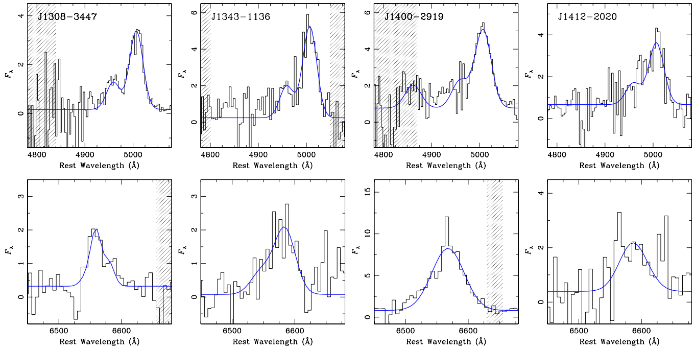
Figure 1. FIRE spectra in the rest frame over the region surrounding H\beta+[O\text{ III}] and H\alpha+[N\text{ II}] . The flux density is in units of 10^{-16} \text{erg s}^{-1} \text{cm}^{-2} \text{\AA}^{-1} . The original spectrum and the model for the emission lines are denoted by a black histogram and a thick blue line, respectively. The position of bright night-sky lines is denoted by the shaded region.
