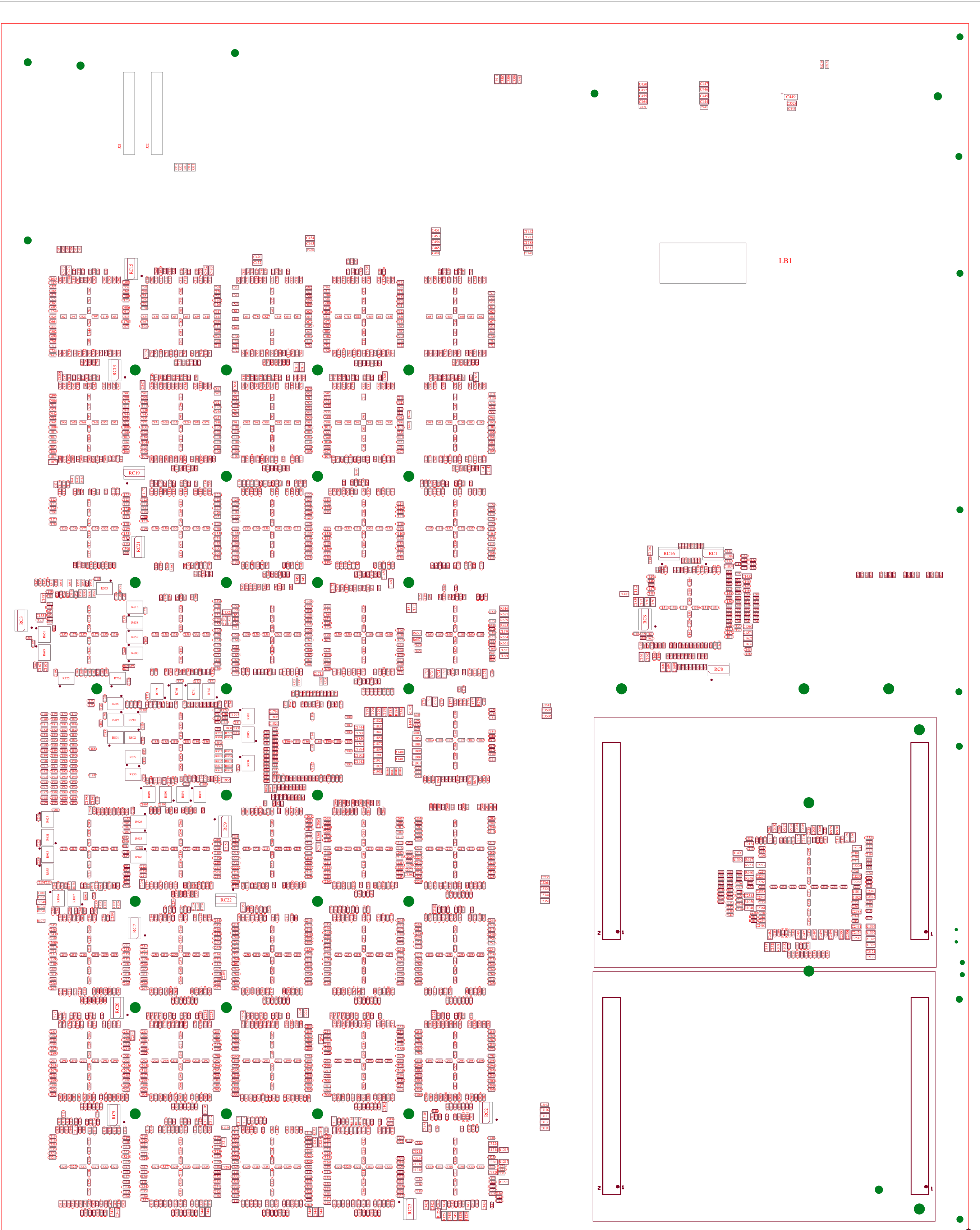
G25040A0005_SB_BottomAssyDrwg_V1.2_Mar18-08
