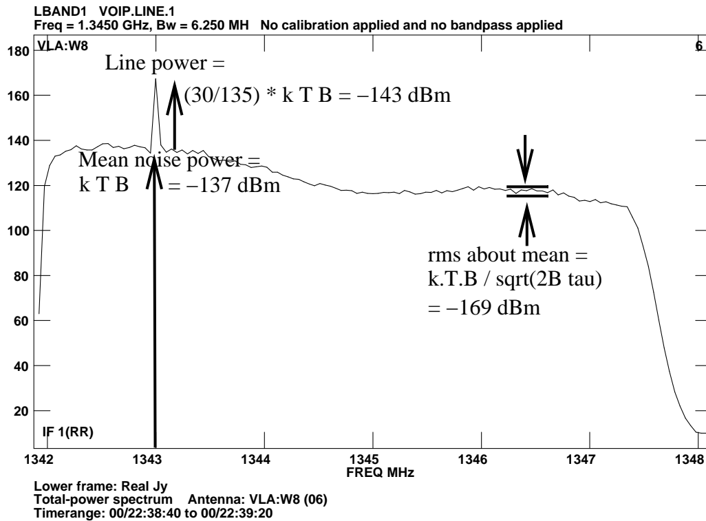
Figure 2: Autocorrelation spectra on ant.6 illustrating the calibration of the received signal in units of the system noise power. The signal of -70dBm in the vertex room leaked into the receiver at -143dBm (shielding of 73dB) at 1343MHz.
