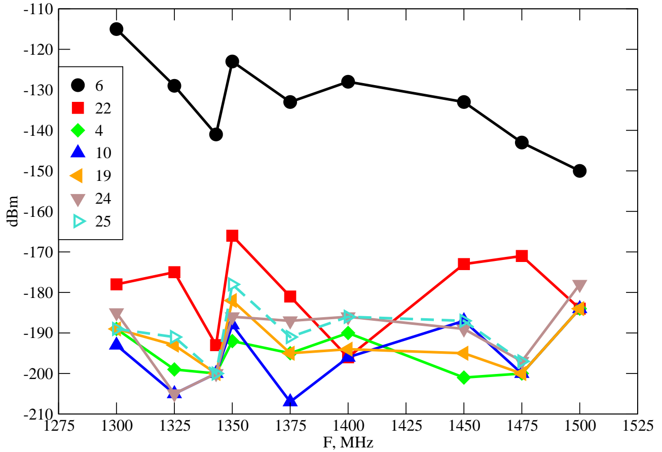
Leakage of VOIP signals from vertex room of VLA ant.6, into receivers on various antennas.
