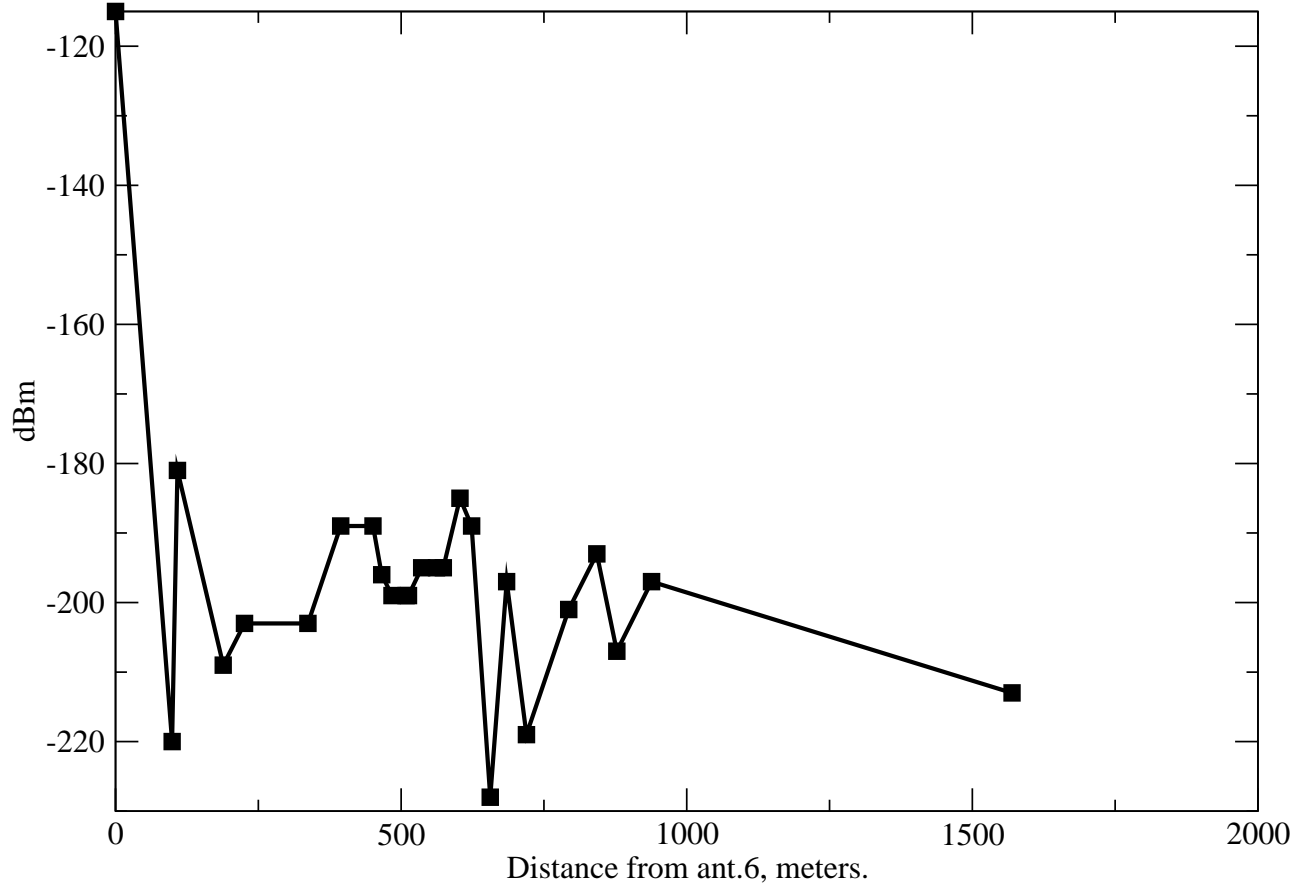
1300 MHz RFI from VOIP in vertex room of VLA ant.6, into receivers at various distances.
