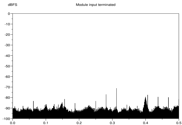
Figure 5: Module noise floor.
