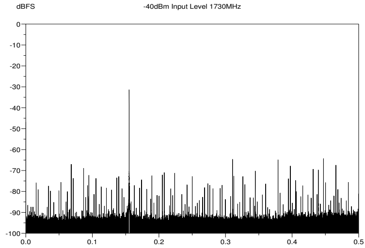
Figure 1: -40dBm input level at 1730MHz.
