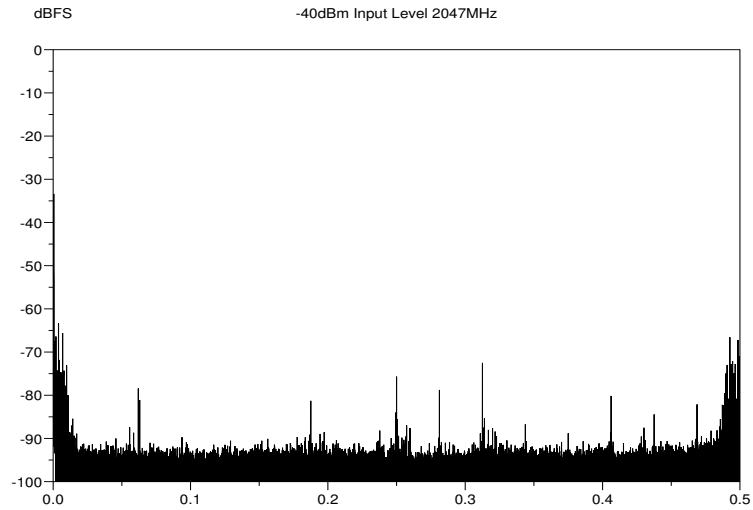
Figure 3: -40dBm input level at 2047MHz.
