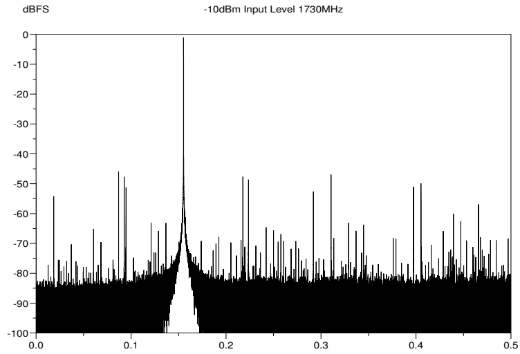
Figure 2: -10dBm input level at 1730MHz.
