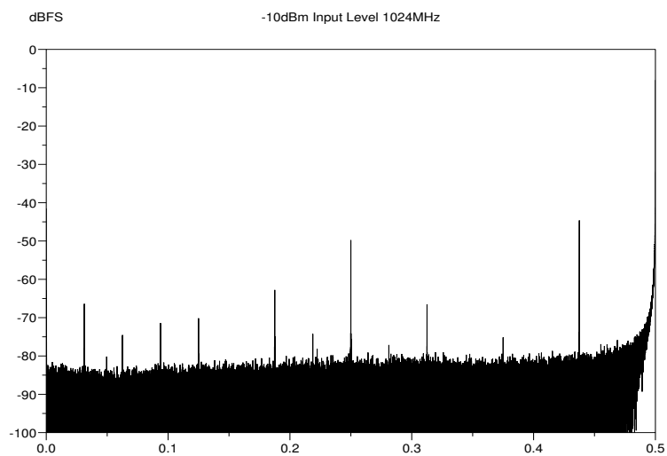
Figure 4: -10dBm signal at Nyquist frequency.
