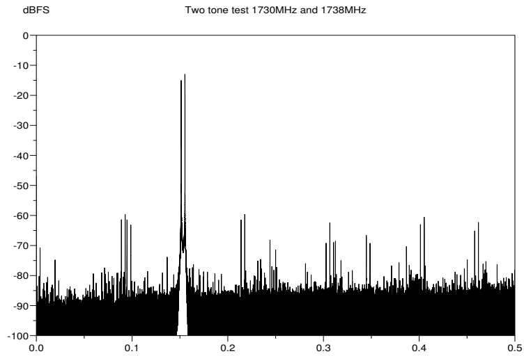
Figure 7: High level two-tone test.
