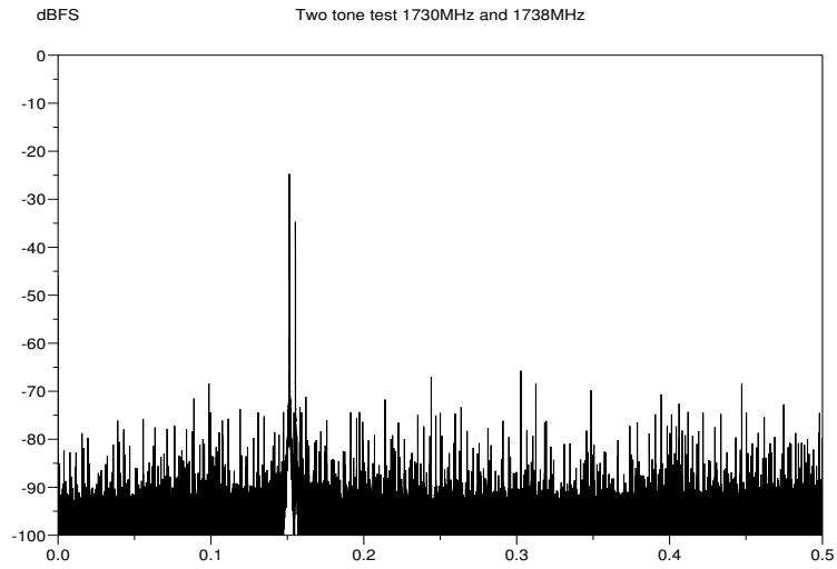
Figure 6: Low level two-tone test.
