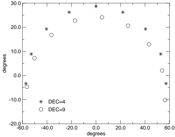
Figure 1: Trajectory of the reference point (declination 4^\circ , labeled by stars) and the point apart in declination and right ascension by 5^\circ (labeled by circles) at the plane zenith angle-azimuth. The array latitude is 34^\circ .
