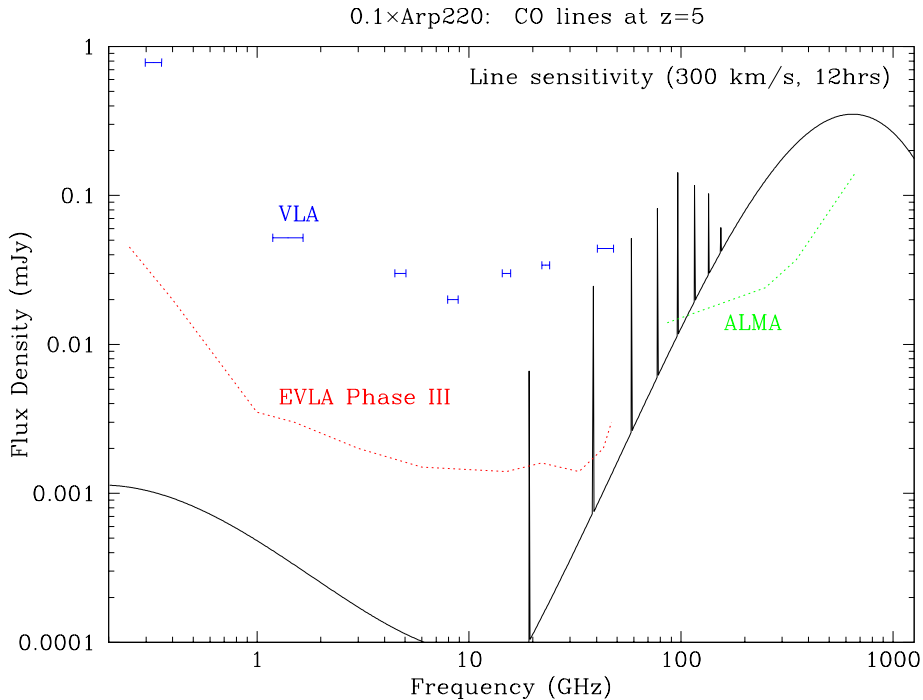
Figure 1. The dotted curves show the ( 1\sigma ) sensitivity to spectral line emission for the VLA, EVLA phase III, and ALMA in 12 hours. The solid curve is the emission spectrum, including continuum and CO lines, for a source with 10% the luminosity of Arp 220 (ie. a source with FIR \sim 10^{11} L_{\odot} ) at z = 5 .
